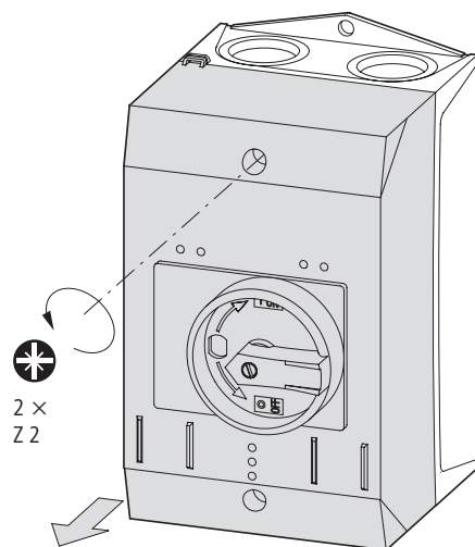
1c CI-K2-PKZ0(-NA)-G(-GR)
