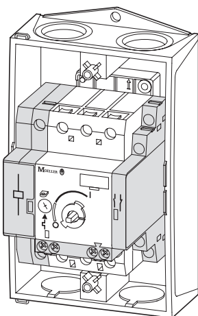
1c CI-K2-PKZ0(-NA)-G(-GR)
