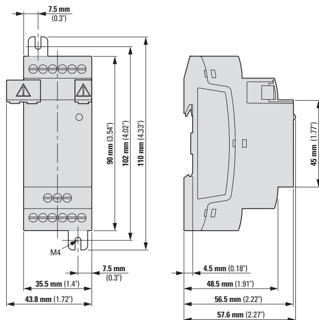
Abb. 298: Abmessungen in mm (Inch)
